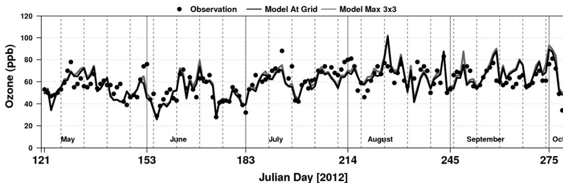
Figure S. 56 Time-series of daily maximum average 8-hour ozone at Auburn Antwoop Road
