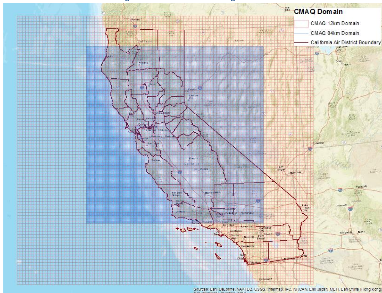
Figure 6-1 CMAQ Modeling Domain
